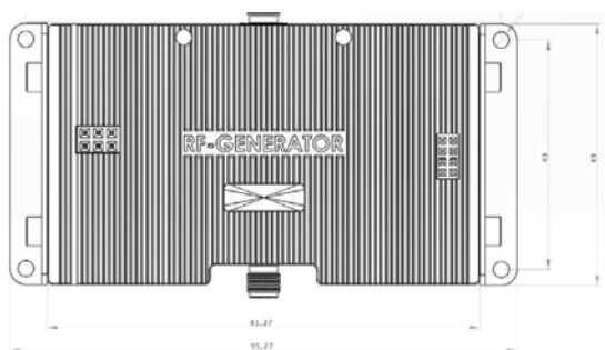
Front view BPSG OEM versions
